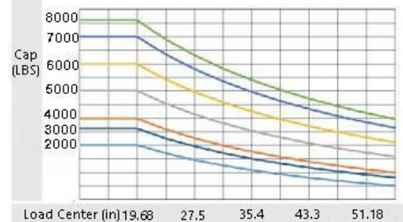
Load curve
