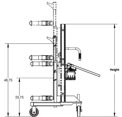
Cylinder Expanded cradle with dual ratchet straps for cylinders and other tall containers
