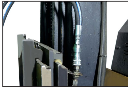
Step 2: Connect quick-connect couplers to forklift auxiliary circuit.
